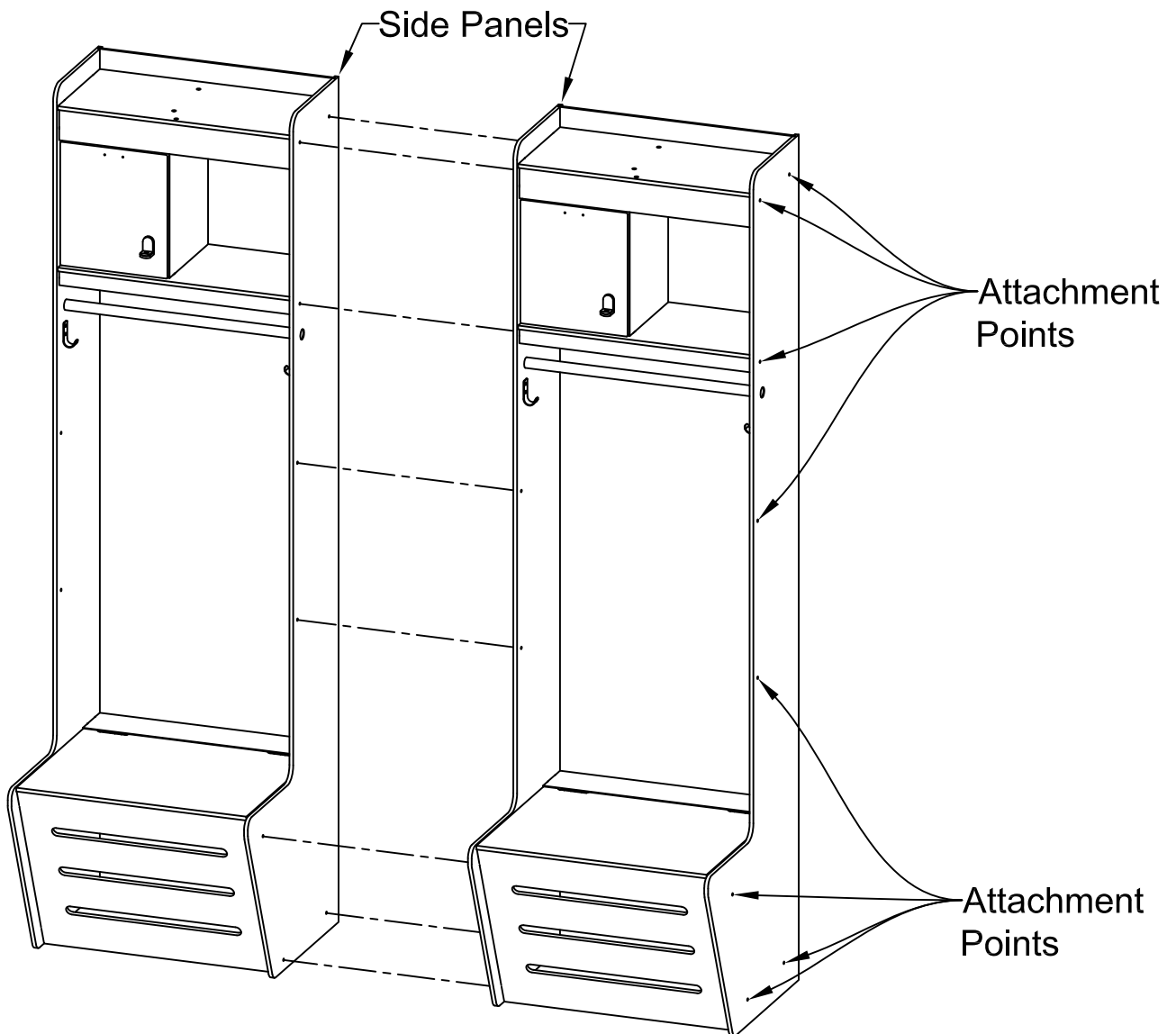
Figure 2.1: Adjacent Locker Installation
