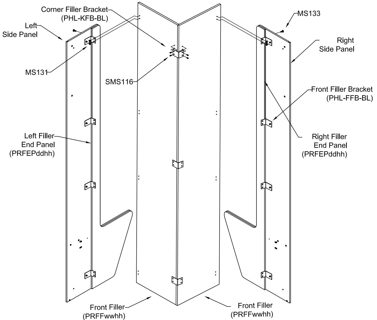
Figure 4.2: Corner Filler
