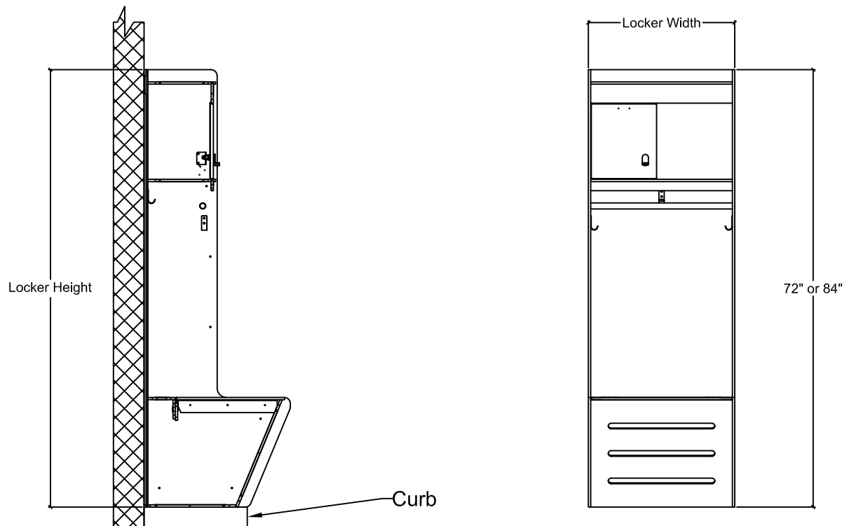
Figure 1.3: Front and Side View
