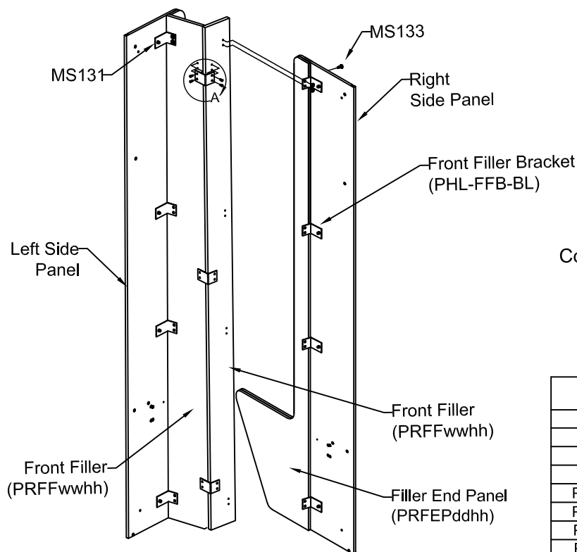
Figure 4.1: Corner Filler
