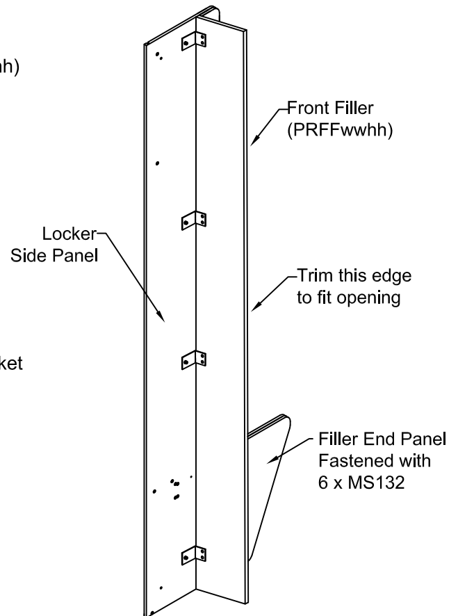
Figure 3.2: Installed Front Filler
