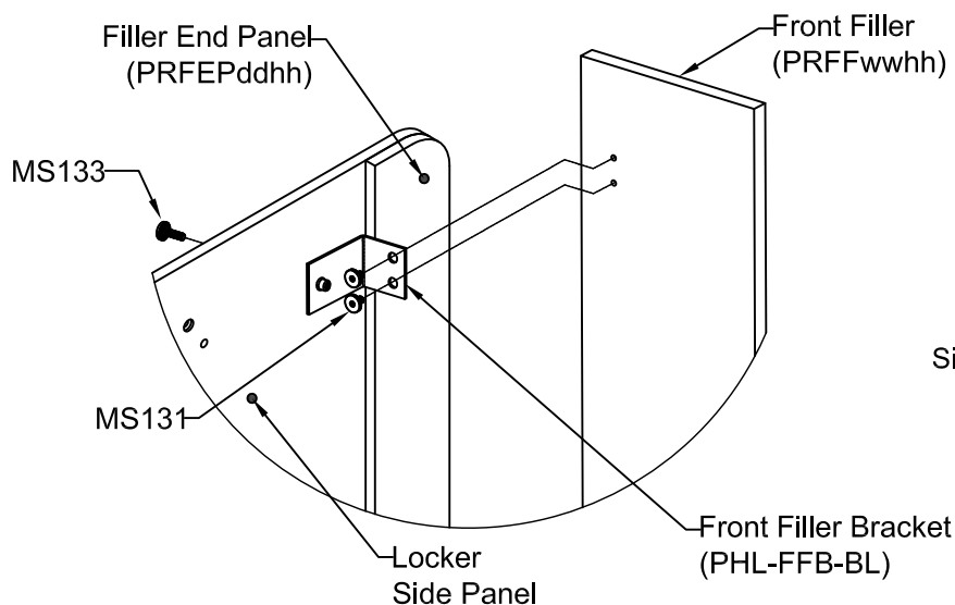
Figure 3.1: Front Filler Brackets
