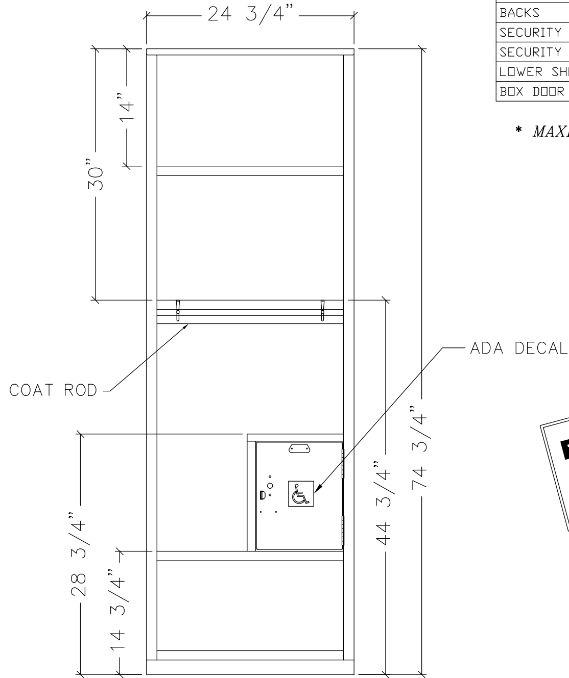
FRONT VIEW
