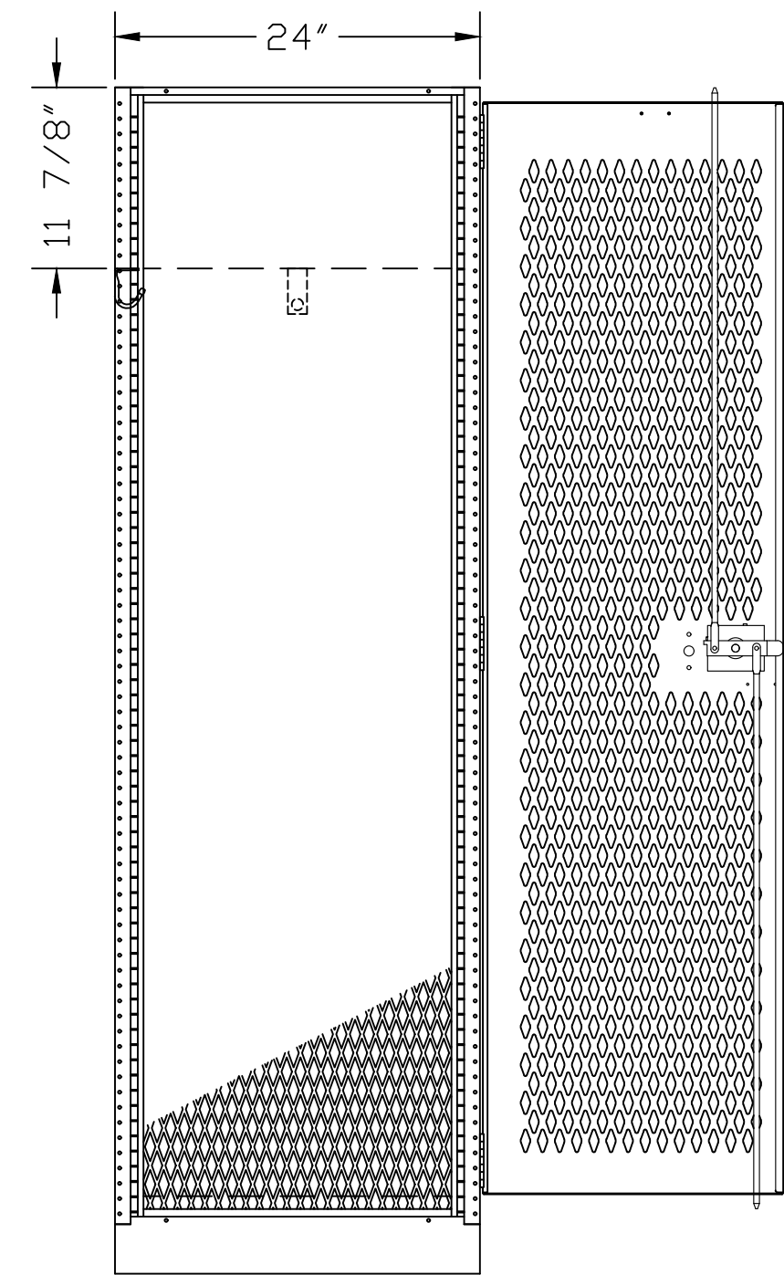
SIDE VIEW
