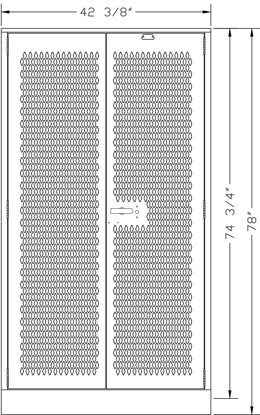
FRONT VIEW
