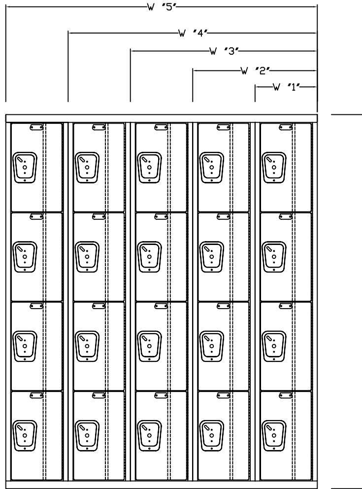
FRONT VIEW
