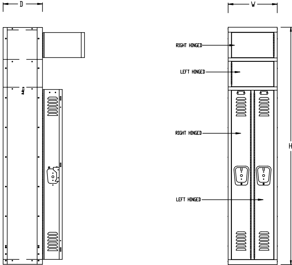
SIDE VIEW
